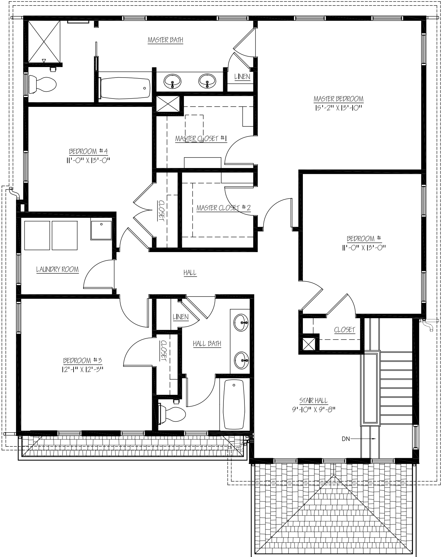
MANOR HOMES AT WESTFIELD MODEL 806 - SECOND FLOOR PLAN
