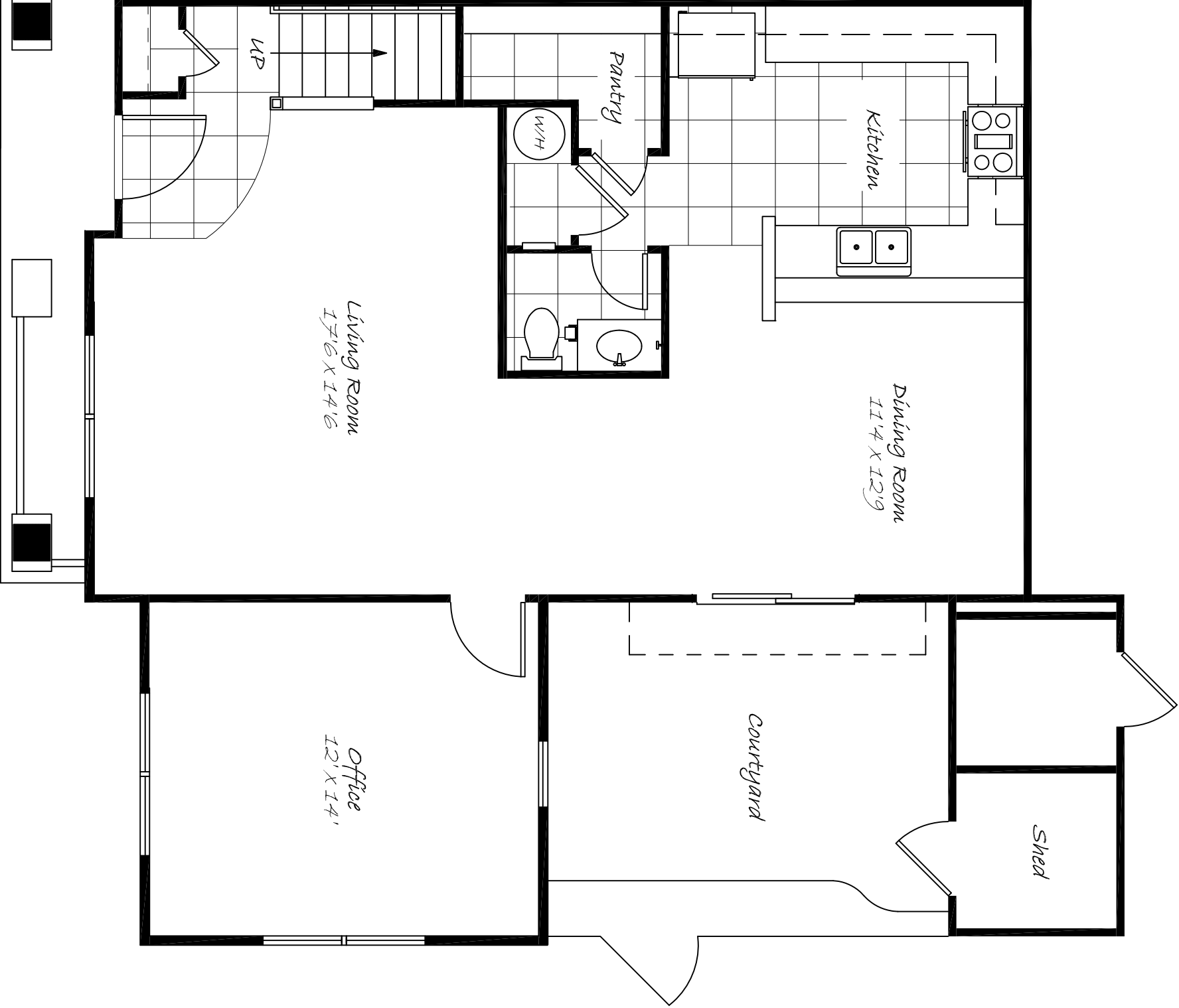
Crofton at Spence Crossing Model #1 First Floor
